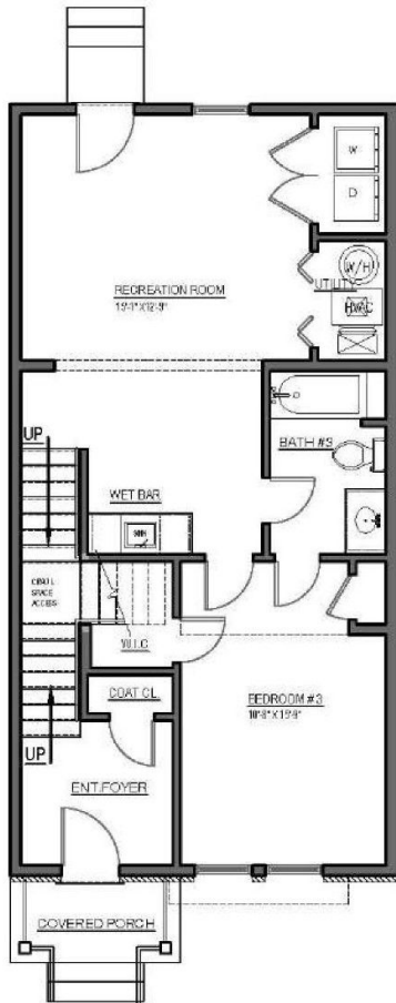
FIRST FLOOR PLAN 800 SF
